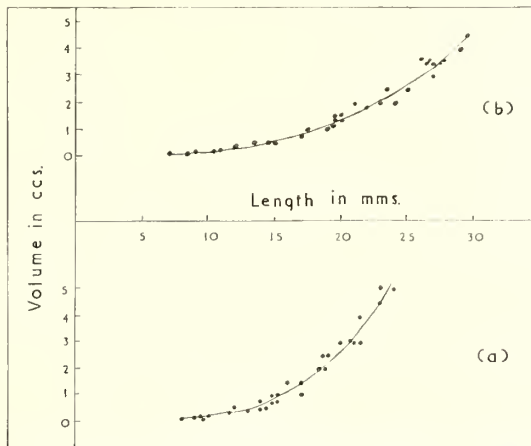
TEXT-FIG. 7. Volume/length relationships in samples of (a) Tetrahynchia and (b) Lobothyris .
